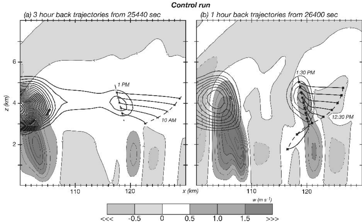
FIG. 9. Control run w (shaded/contoured) and q_c (contoured) fields with backward trajectories started at time shown: (a) fields at 25 440 with q_c contour interval of 0.05 g kg^{-1} ; (b) fields at 26 400 s with q_c contour interval 0.2 g kg^{-1} . Contours for negative values are dashed. Please note that cloud water contour intervals are not the same and differ from that employed in Fig. 1.
