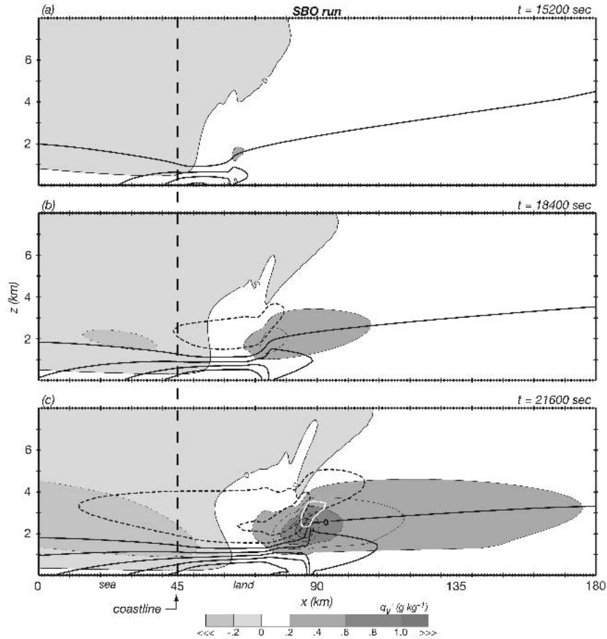
FIG. 3. SBO run fields of perturbation vapor mixing ratio ( q'_v , shaded) and horizontal (cross-shore) velocity ( u , 2 \text{ m s}^{-1} contours). Contours for negative values are dashed. Thick white contour encloses saturated region.
