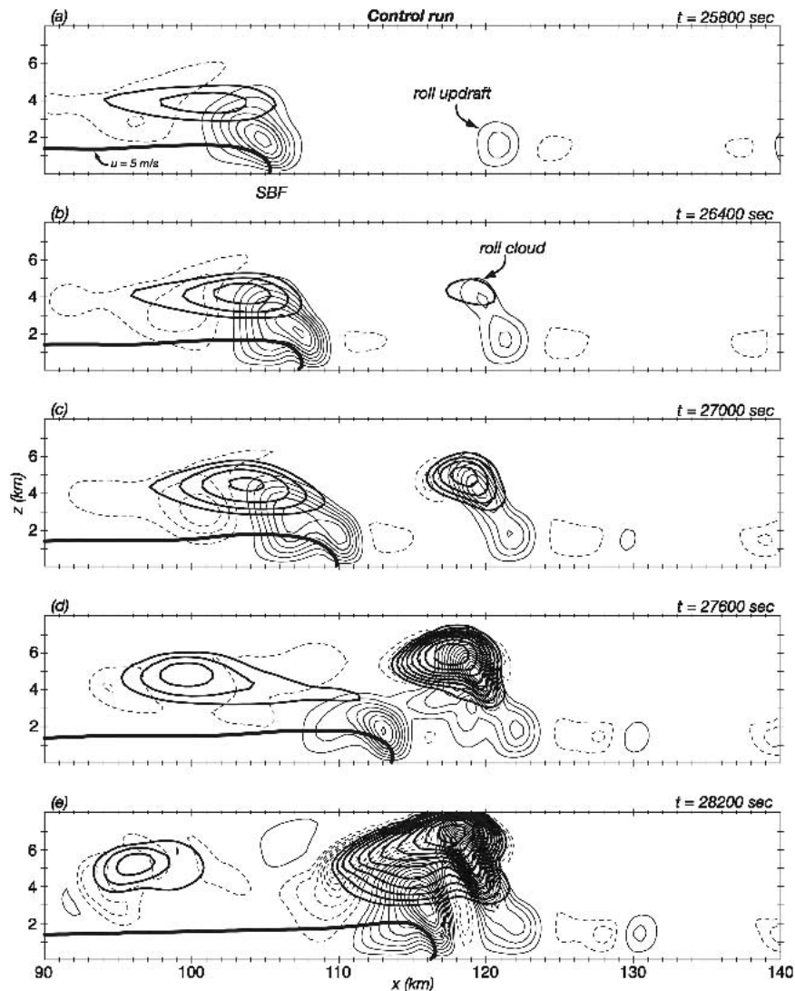
FIG. 1. Control run fields of vertical velocity ( w , 0.5 \text{ m s}^{-1} , thin contours) and cloud water mixing ratio ( q_c , 0.5 \text{ g kg}^{-1} , thick contours), averaged in the along-coastal direction. The 5 \text{ m s}^{-1} contour of ground-relative cross-shore horizontal velocity, a proxy for the marine air boundary, is superposed; its leading edge is the sea-breeze front (SBF). Contours for negative values are dashed; only a portion of the domain is shown. Times shown relative to sunrise (0600 LST).
