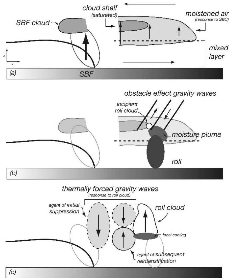
FIG. 13. Schematic depiction of SBC and roll-related influences leading to deep convection ahead of the SBF in the control run.
