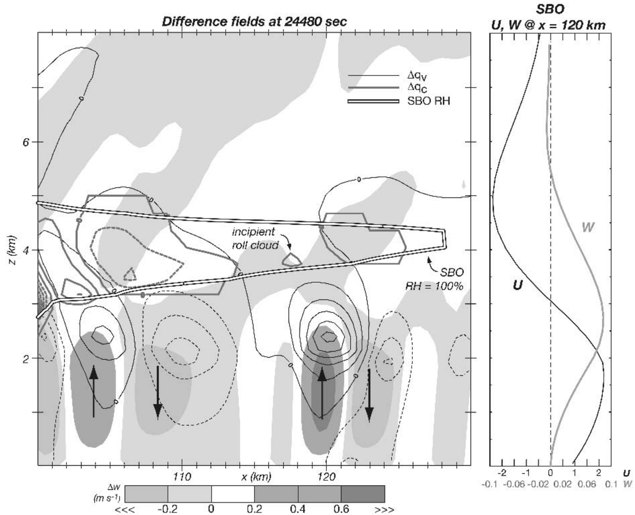
FIG. 7. Control-SBO difference fields at 24 480 s. Shown are vertical velocity \Delta w (shaded), water vapor mixing ratio ( \Delta q'_v , 0.1 \text{ g kg}^{-1} , thin black contours), and cloud water mixing ratio ( \delta q_c , 0.01 \text{ g kg}^{-1} , thick gray contours) difference fields. Contours for negative values are dashed. Saturated region from the SBO run is marked. Vertical profiles of u and w from the SBO run at a designated location reveal the background field upon which the control run's rolls are superposed.
