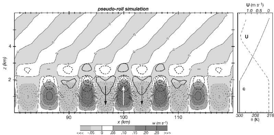
FIG. 6. Pseudoroll simulation employing a maintained streamfunction field with weak forcing to generate roll-like circulations, showing vertical velocity w (shaded/contoured) and perturbation potential temperature \theta' (0.005 K contours). Contours for negative values are dashed. Profiles of u and \theta at right resemble those present inland of the SBF in the early afternoon. (Vertical shear within the mixed layer has been neglected for simplicity.)
