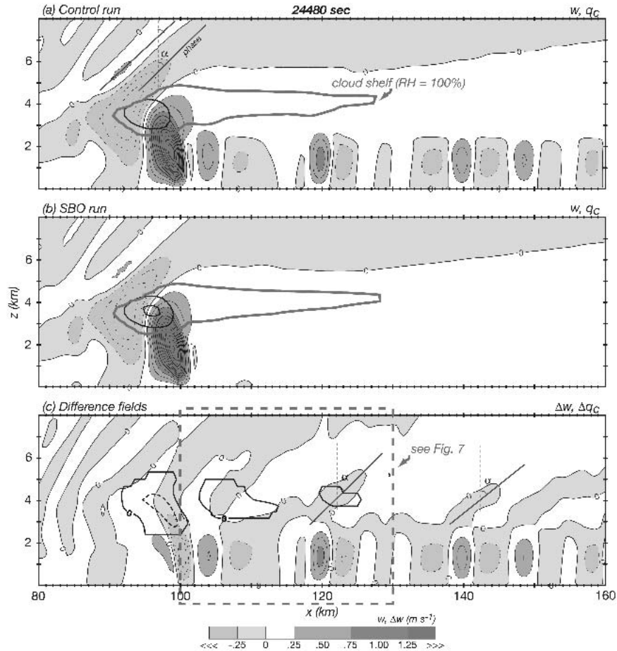
FIG. 5. Control, SBO, and control-SBO difference fields at 24 480 s. (a), (b) Vertical velocity w (shaded and contoured) and cloud water q_c ( 0.5 \text{ g kg}^{-1} , thick contours) with saturated region identified. (c) vertical velocity and cloud water difference fields \Delta w and \Delta q_c . Contour interval for \Delta q_c is 0.1 \text{ g kg}^{-1} . Contours for negative values are dashed. Figure 7's subdomain is delineated.
