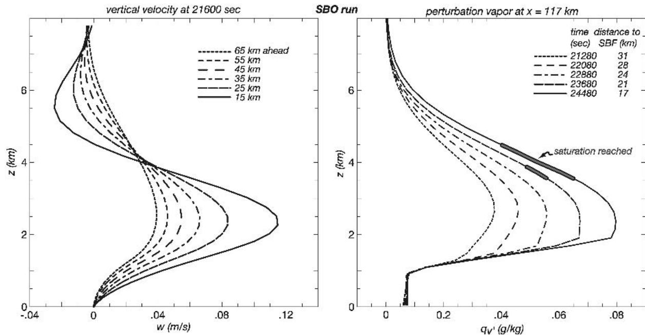
FIG. 4. Vertical profiles of along-coast-averaged quantities from the SBO run: (a) vertical velocity w at 21 600 s for specified distances ahead of the SBF; (b) perturbation vapor q_v' profiles at various times for a selected location ( x = 117 km; see Figs. 2 and 3). Thick gray lines mark height levels where saturation has been achieved.
