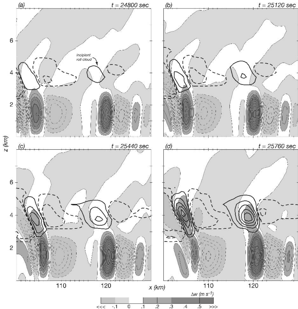
FIG. 8. Control-SBO vertical velocity ( \Delta w , shaded/contoured) and cloud water ( \Delta q_c ) difference fields; \Delta q_c contours selected for inclusion are the 0.01, 0.05, 0.09, 0.13, and 0.17 \text{g kg}^{-1} isolines, in addition to the -0.0001 and -0.025 \text{ g kg}^{-1} values. Contours for negative values are dashed.
