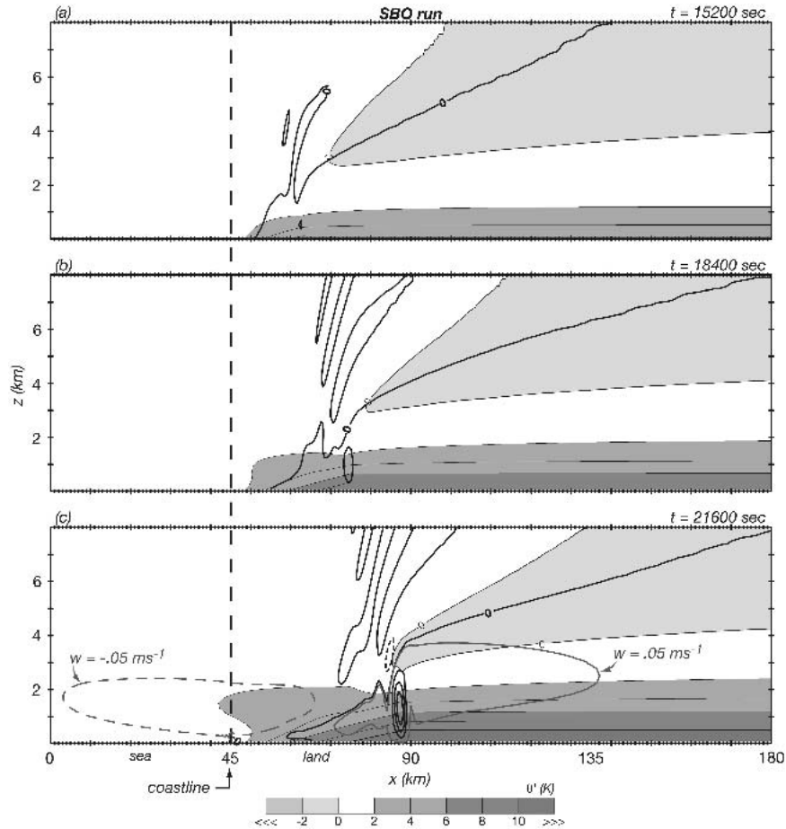
FIG. 2. SBO run along-coastal-averaged fields of perturbation potential temperature ( \theta' , shaded) and vertical velocity ( w , 0.5 \text{ m s}^{-1} contours). Perturbations are relative to the initial state. Contours for negative values are dashed. Selected contours of w = \pm 0.05 \text{ m s}^{-1} are superposed.
