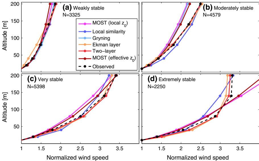
Fig. 5 Modelled and observed mean wind-speed profiles for the different stability regimes
