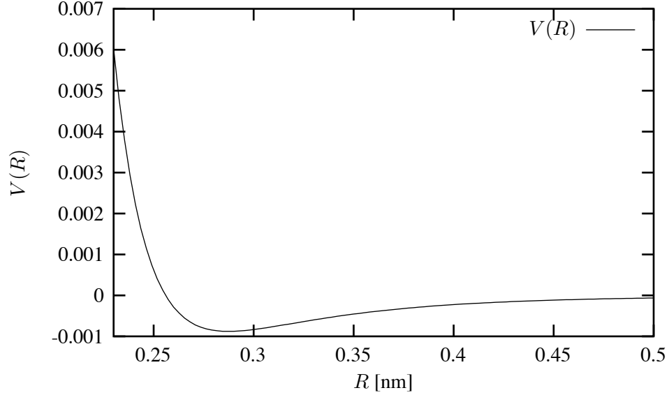
Figure 11.5: Plot for the Van der Waals interaction between helium atoms. The equilibrium position is r_0 = 0.287 nm.
