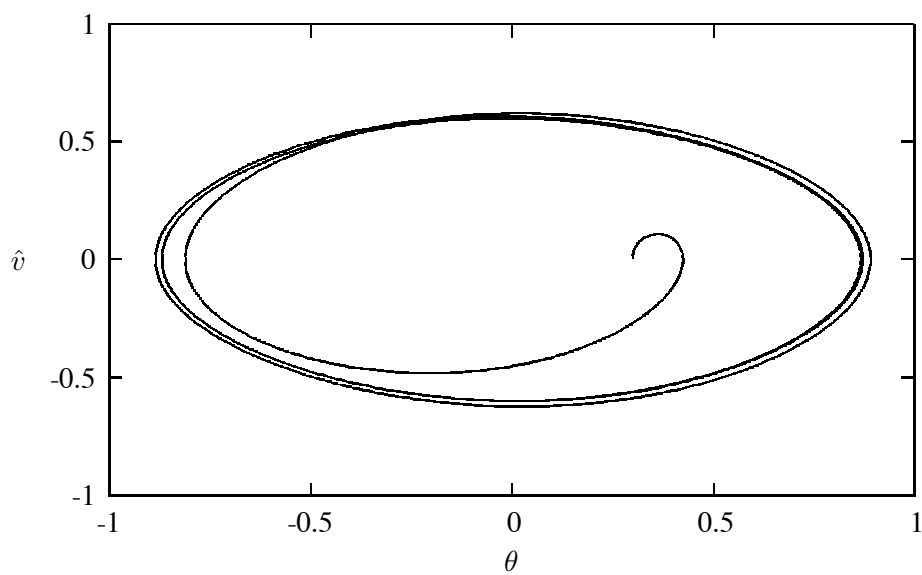
Figure 13.8: Phase-space curve with Q = 2 , \hat{\omega} = 2/3 and \hat{A} = 0.5 . The mass of the pendulum is set equal to 1 kg and its length l = 1 m.. The initial velocity is \hat{v}_0 = 0 and \theta_0 = 0.3 .
