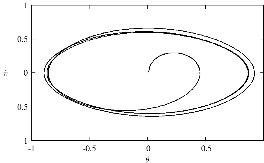
Figure 13.6: Phase-space curve of a linear damped pendulum with Q = 2 , \hat{\omega} = 2/3 and \hat{A} = 0.5 . The initial velocity is \hat{v}_0 = 0 and \theta_0 = 0.01 .
