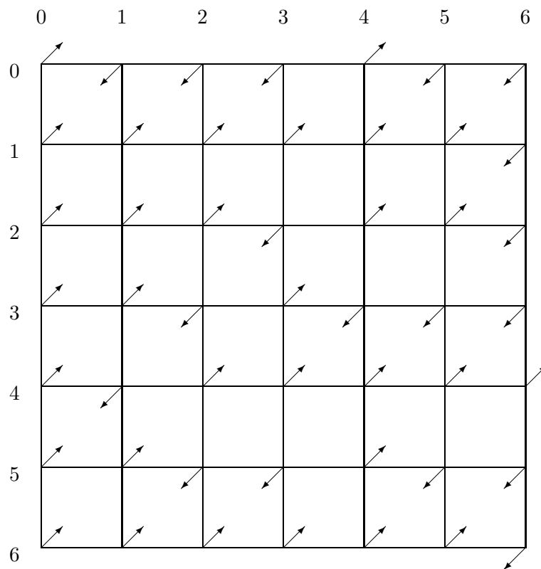
Figure 10.4: Example of a two-dimensional 7 \times 7 lattice with spins pointing either up or down. The variable spin_matrix [0][1] takes the value +1 while spin_matrix [6][0] is -1.
