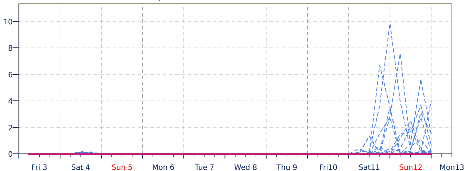
Ensemble members of Total Precipitation (mm/6h)
