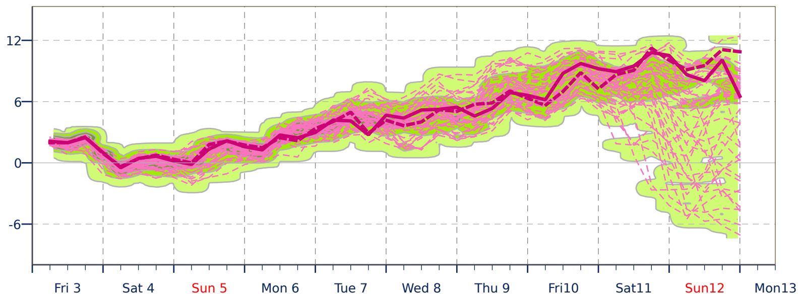
Temperature at 850 hPa - Probability for 1°C intervals
