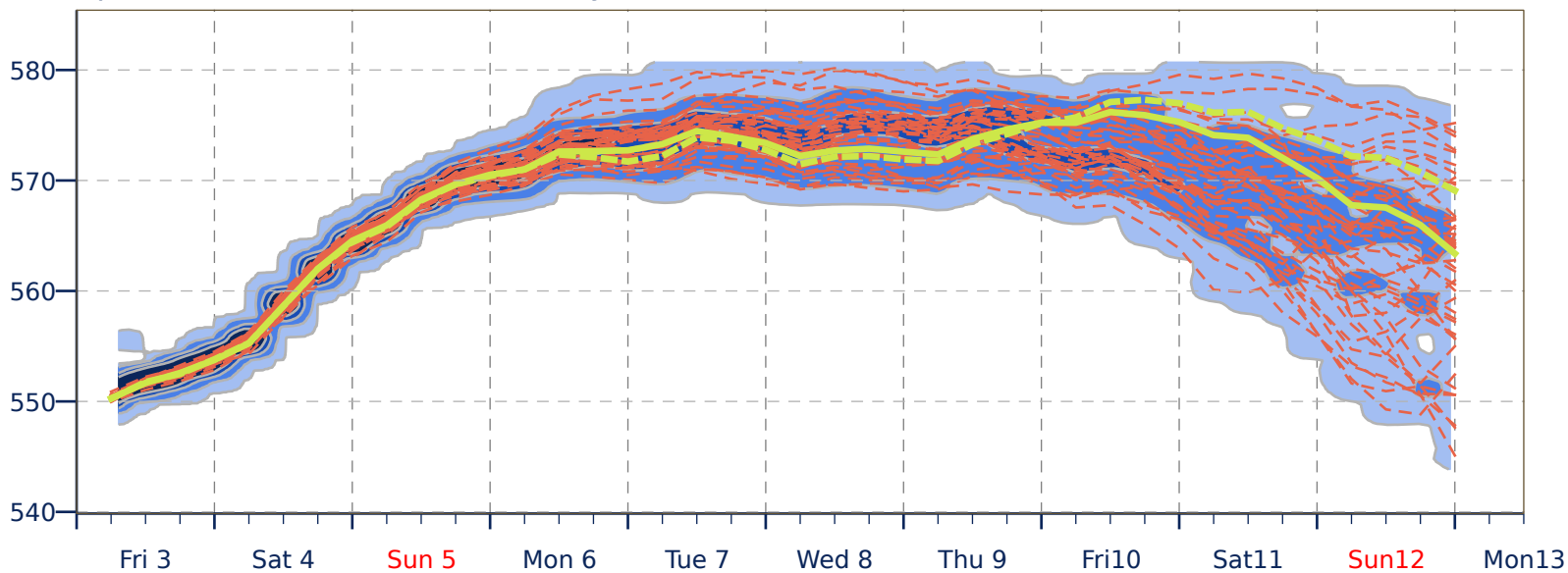
Geopotential at 500 hPa -- Probability for 2.5dam intervals
