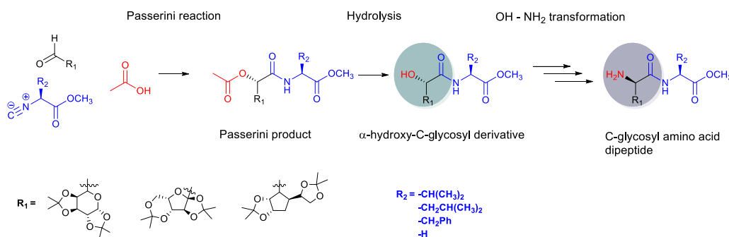
Figure 1. Synthesis to C-glycosyl amino acid derivatives by post-condensation modification of Passerini products.
