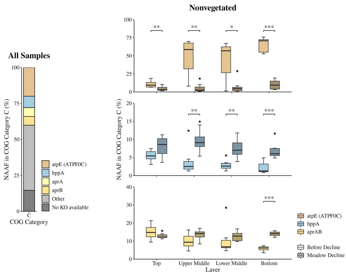
Fig. 4 Proportion of the most abundant (> 3%) KEGG KO entries within the functional COG category C (energy production and conversion) in all samples and changes in the proportion of the same entries in each layer at the nonvegetated site before and during the decline of the C. nodosa meadow in the Bay of Saline. The proportion was calculated using the NAAF. The asterisks indicate the level of statistical significance: * p < 0.05 , ** p < 0.01 , and *** p < 0.001 , while the dots represent outliers
