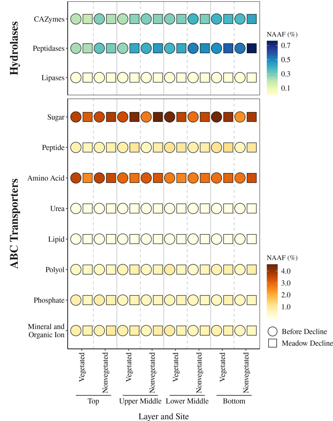
Fig. 5 Median proportion of groups of hydrolases and ABC transporters in sediment layers at the vegetated and nonvegetated site before and during the decline of the C. nodosa meadow in the Bay of Saline. The proportion was calculated using the NAAF
