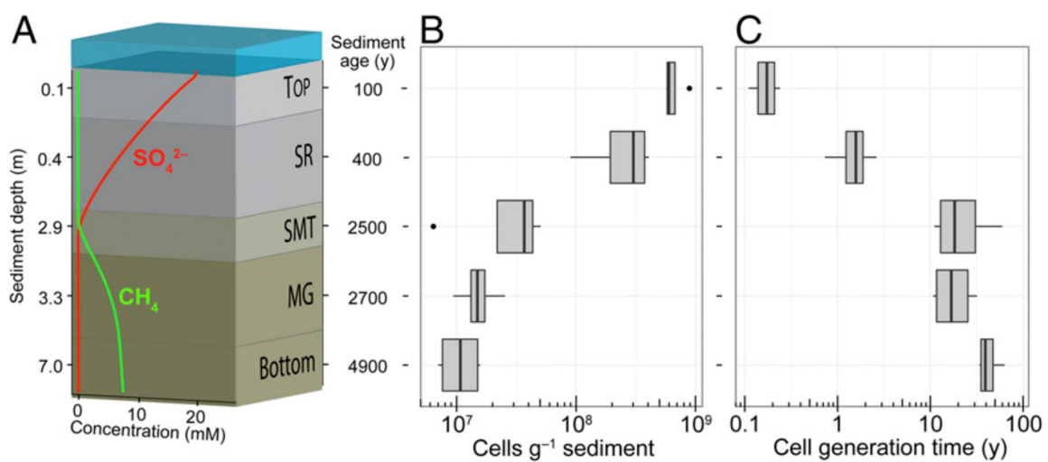
Figure 2. The vertical biogeochemical zonation (A) and the corresponding distribution of microbial cell abundances (B) and generation times (C) in sediments. Biogeochemical zones: Top, surface sediment; SR, upper sulphate-rich sediment; SMT, sulphate–methane transition zone; MG, methanogenic sediment; Bottom, deep methanogenic zone. From Starnawski et al. (2017).
