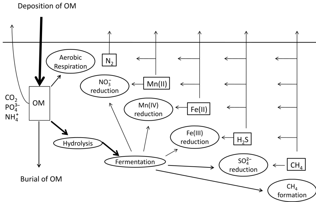
Figure 4. Conceptual model of the degradation of organic matter in marine sediments. High-molecular-weight organic matter is converted into smaller substrates by hydrolysis and fermentation. These products are respired with the most energetically favourable terminal electron acceptors in the following order of utilisation: oxygen ( O_2 ), nitrate ( NO_3^- ), manganese [ Mn(IV) ] and iron [ Fe(III) ] oxides, sulphate ( SO_4^{2-} ), and carbon dioxide ( CO_2 ). Manganese [ Mn(II) ], iron [ Fe(II) ], sulphide ( H_2S + HS^- + S^{2-} ), and methane ( CH_4 ) are produced and can be oxidised after diffusing upwards. Modified from Middelburg and Levin (2009).
