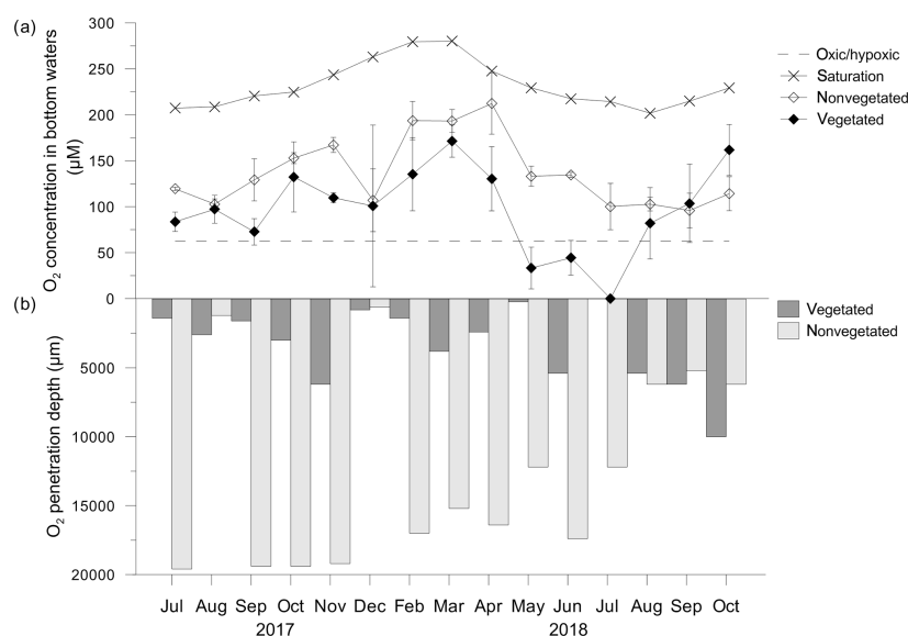
Figure 6. (a) Oxygen ( O_2 ) concentrations in bottom waters in, and (b) O_2 penetration depths above, vegetated and nonvegetated sediment. O_2 at the saturation level was calculated according to the temperature and salinity measured in seawater on the sampling dates; O_2 at the hypoxic frontier ( \sim 62.5 \mu M ) was taken from Vaquer-Sanyer and Duarte (2008).
