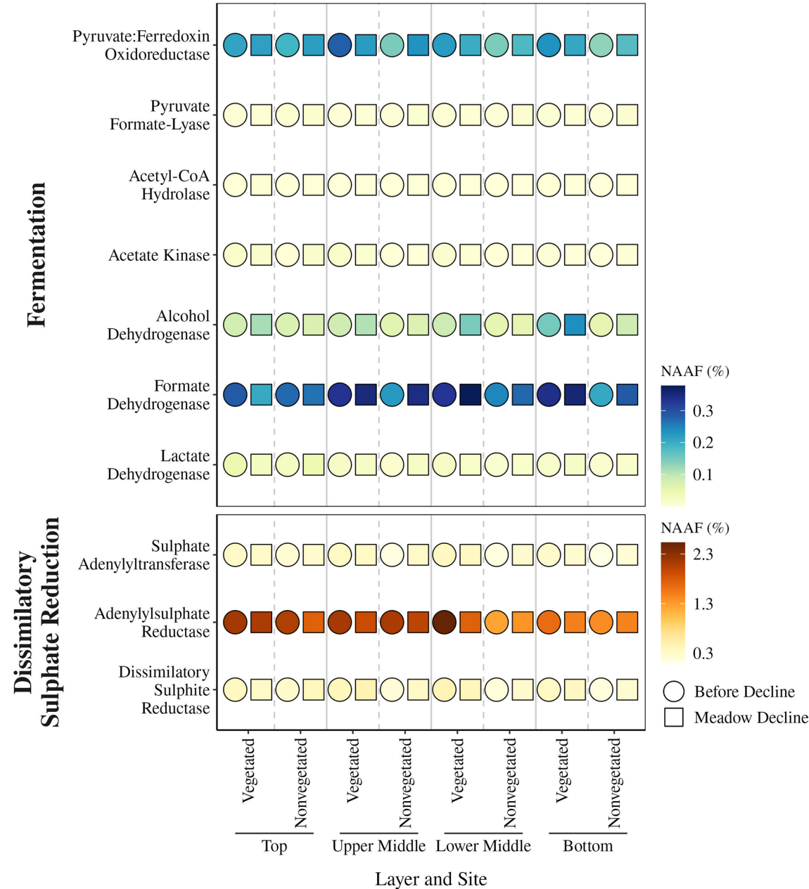
Fig. 6 Median proportion of enzymes involved in mediating various fermentation products and dissimilatory sulphate reduction in sediment layers at the vegetated and nonvegetated site before and during the decline of the C. nodosa meadow in the Bay of Saline. The proportion was calculated using the NAAF
